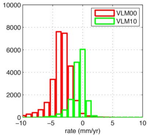
Figure 8. Histograms of Vertical Displacement Rates for All Scatterers Within the Delta for the VLM00 and VLM10 Solutions
